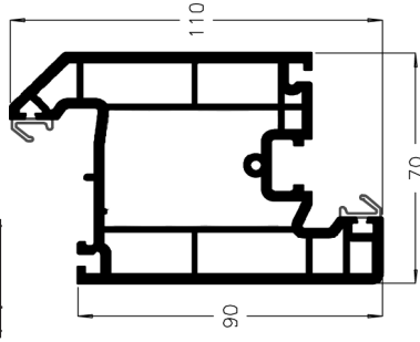
P10510 110mm Door Sash (open in)
