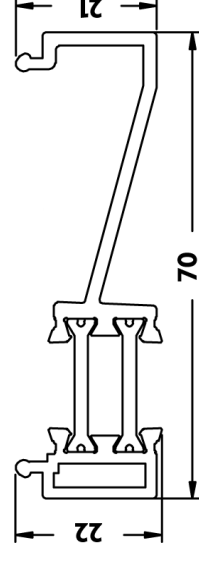
DV172 22mm Add on
