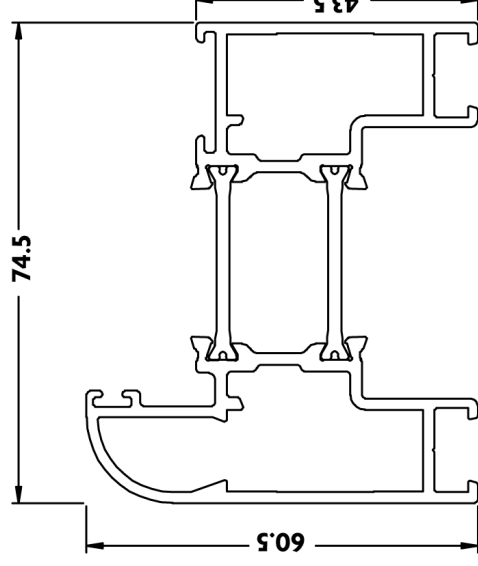
DV26 Rounded Sash
