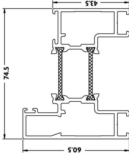
DV23 Flat Sash
