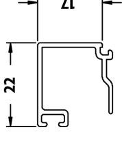
DV67 28mm Square Bead
